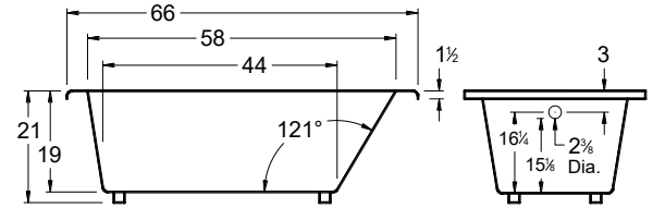
All bathtub dimensions are ± 1/2".
