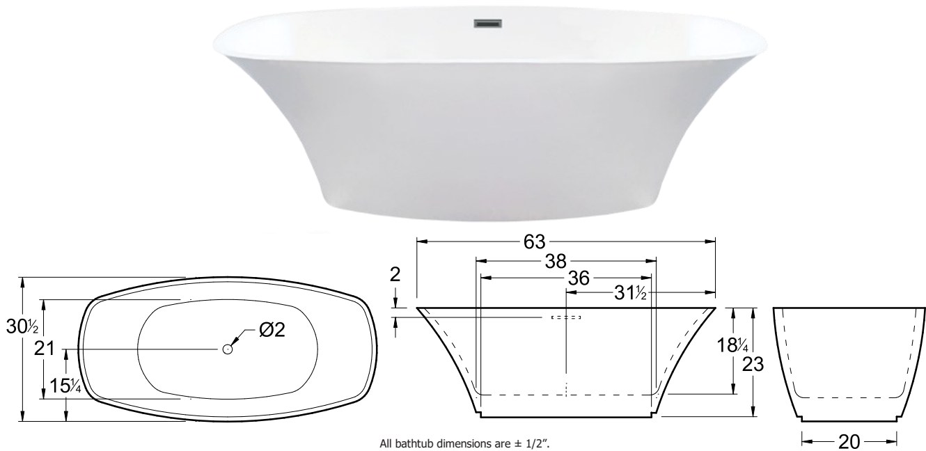
All bathtub dimensions are \pm 1/2 ".
